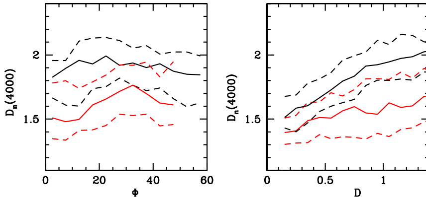
Figure 16: D_n(4000) is plotted as a function of \Phi (for AGN lying above the Kewley et al line) and D for weak AGN (black) and for strong AGN (red). The solid lines indicate the median and the dashed lines the 16-84 percentiles of the 1/V_{max} weighted distribution.
